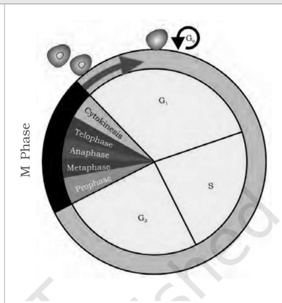
Fig. 10.1 - A diagrammatic view of cell cycle indicating formation of two cells from one cell.
